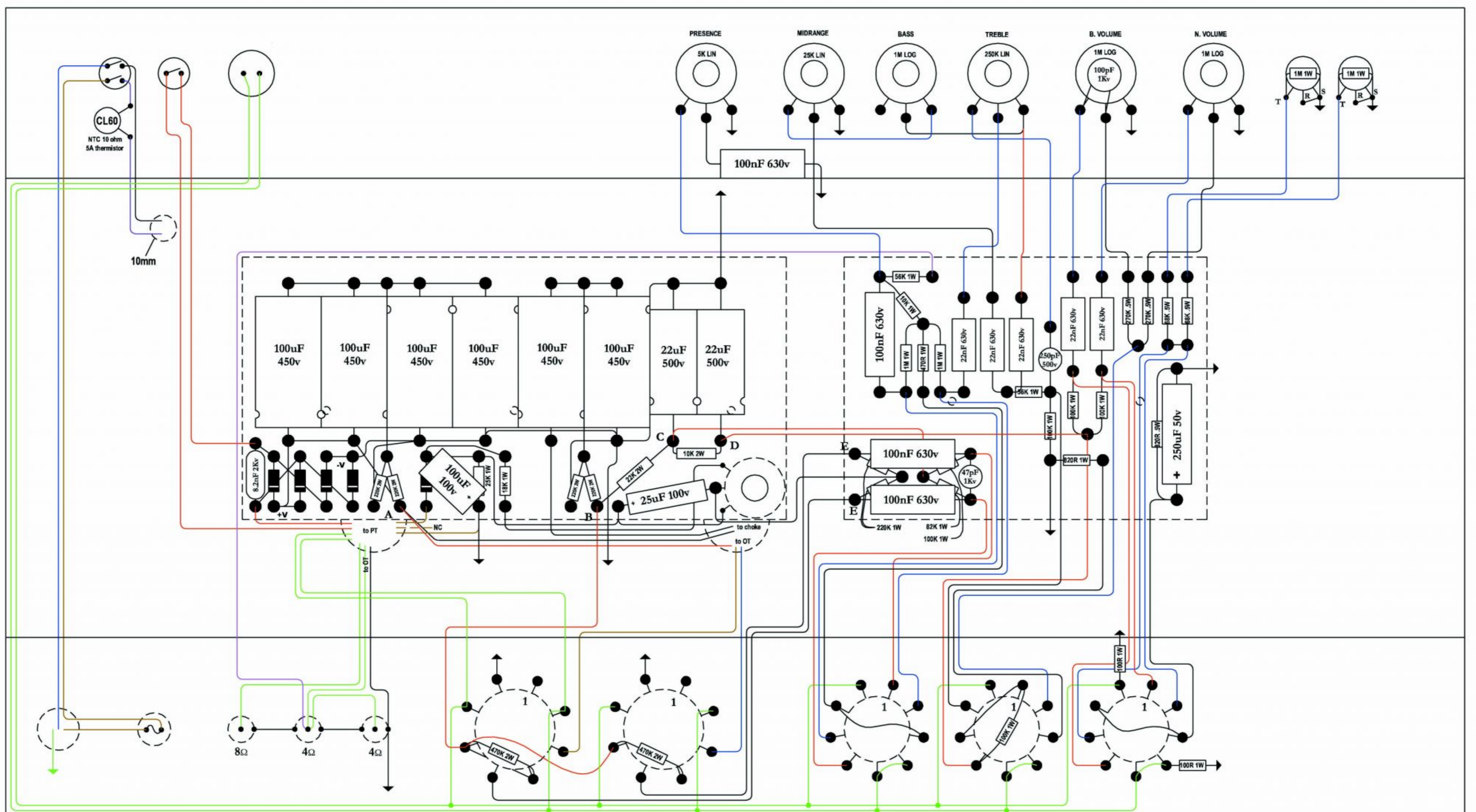
Hot Rod Deville Chassis - 5F6A w/ HRDv PS & OT- 240V
